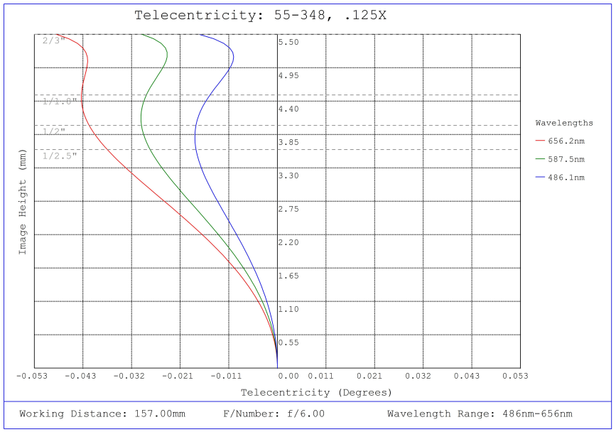
#55-348, 0.125X, 2/3" GoldTL™ Telecentric Lens, Telecentricity Plot
