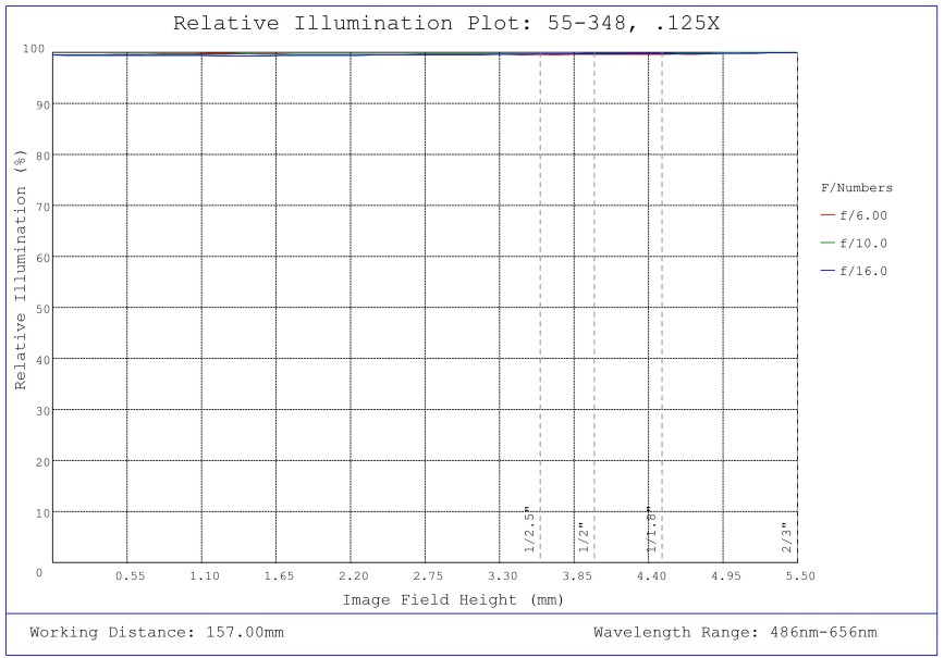
#55-348, 0.125X, 2/3" GoldTL™ Telecentric Lens, Relative Illumination Plot
