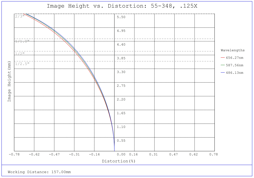
#55-348, 0.125X, 2/3" GoldTL™ Telecentric Lens, Distortion Plot
