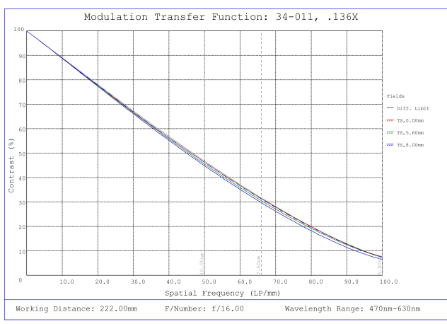
#34-011, 0.136X, 1" C-Mount TitanTL® Telecentric Lens, Modulated Transfer Function (MTF) Plot, 222mm Working Distance, f16
