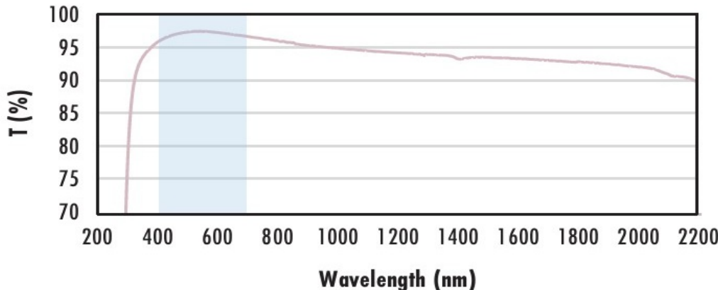
N-BK7 with \text{MgF}_2 Coating Typical Transmission
