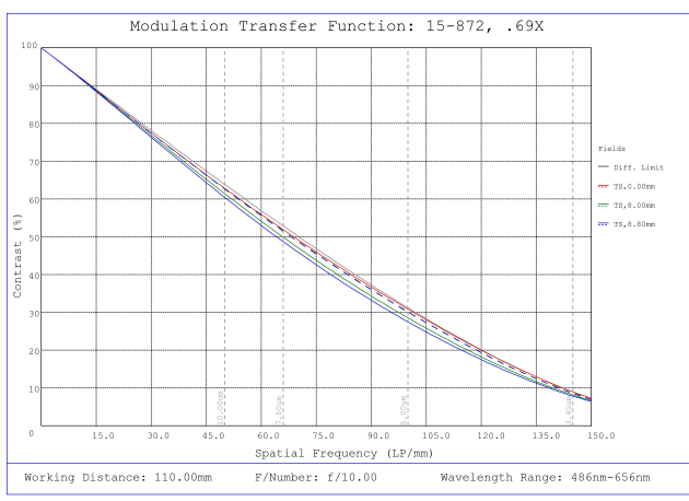
#15-872, 0.69X CobaltTL Telecentric Lens, Modulated Transfer Function (MTF) Plot, 110mm Working Distance, f10
