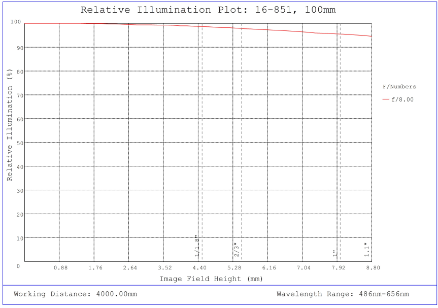
#16-851, 100mm, f/8 Athermal Lens, Relative Illumination Plot
