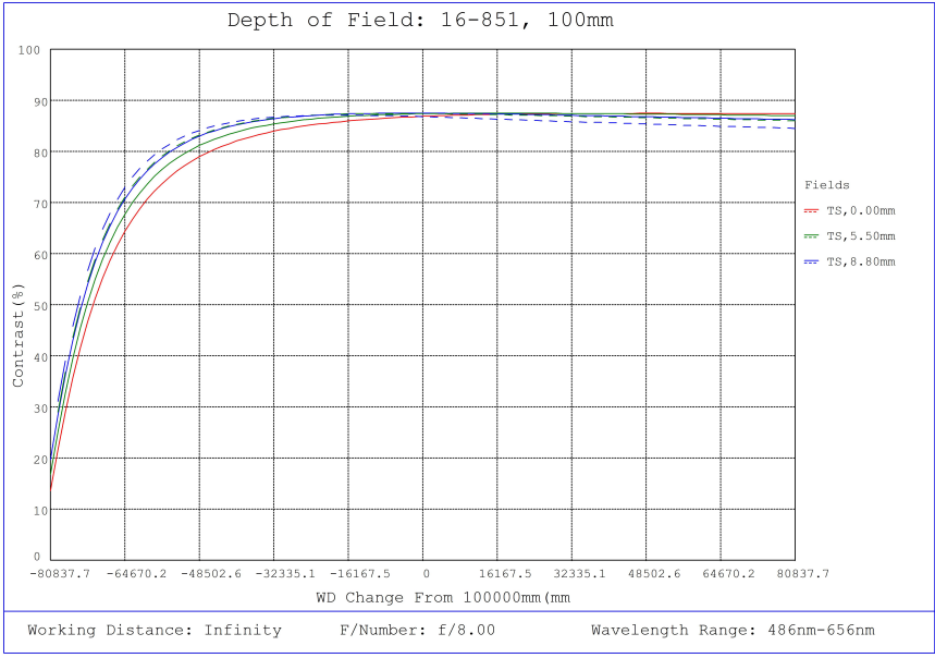
#16-851, 100mm, f/8 Athermal Lens, Depth of Field Plot, 10000mm Working Distance, f8
