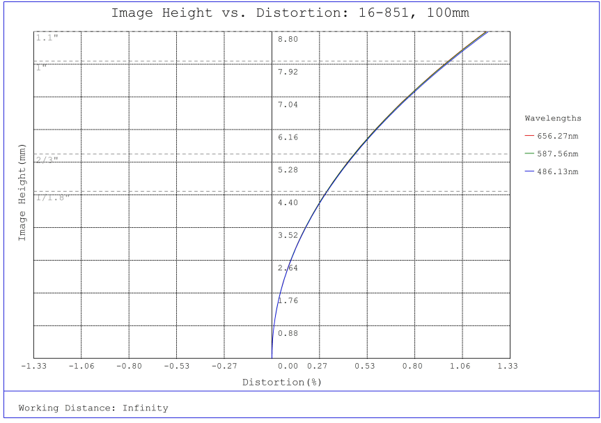
#16-851, 100mm, f/8 Athermal Lens, Distortion Plot
