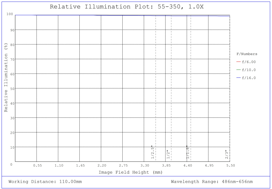
#55-350, 1.0X 2/3" GoldTL™ Telecentric Lens, Relative Illumination Plot
