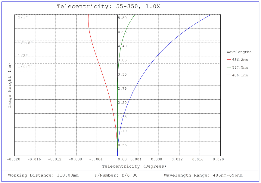
#55-350, 1.0X 2/3" GoldTL™ Telecentric Lens, Telecentricity Plot
