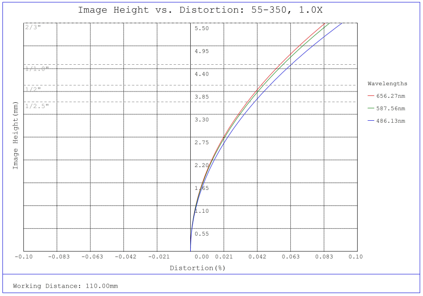
#55-350, 1.0X 2/3" GoldTL™ Telecentric Lens, Distortion Plot
