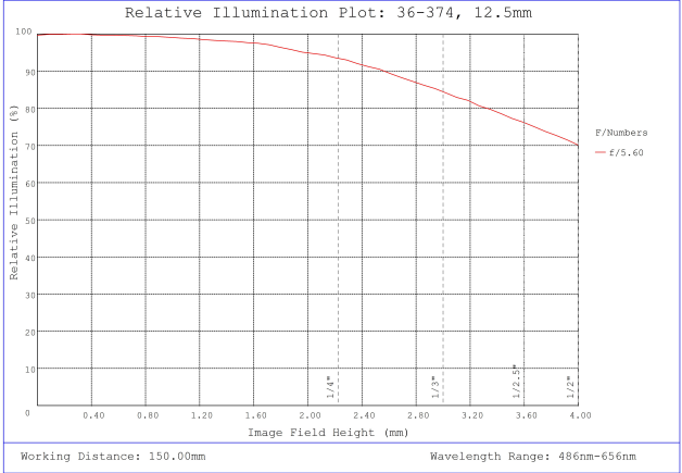
#36-374, 12.5mm FL f/5.6, Rugged Blue Series M12 Lens, Relative Illumination Plot
