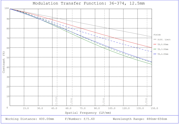
#36-374, 12.5mm FL f/5.6, Rugged Blue Series M12 Lens, Modulated Transfer Function (MTF) Plot, 400mm Working Distance, f5.6
