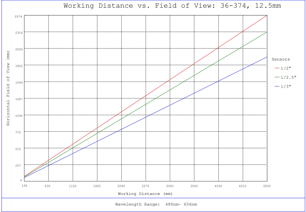
#36-374, 12.5mm FL f/5.6, Rugged Blue Series M12 Lens, Working Distance versus Field of View Plot
