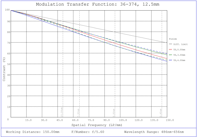
#36-374, 12.5mm FL f/5.6, Rugged Blue Series M12 Lens, Modulated Transfer Function (MTF) Plot, 150mm Working Distance, f5.6
