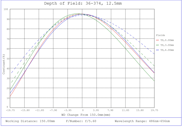
#36-374, 12.5mm FL f/5.6, Rugged Blue Series M12 Lens, Depth of Field Plot, 150mm Working Distance, f5.6
