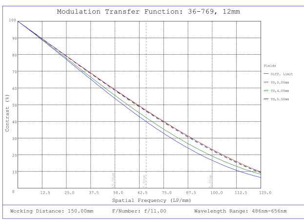
#36-769, 12mm f/11, 150-500mm Primary WD, HRi Series Fixed Focal Length Lens, Modulated Transfer Function (MTF) Plot, 150mm Working Distance, f11
