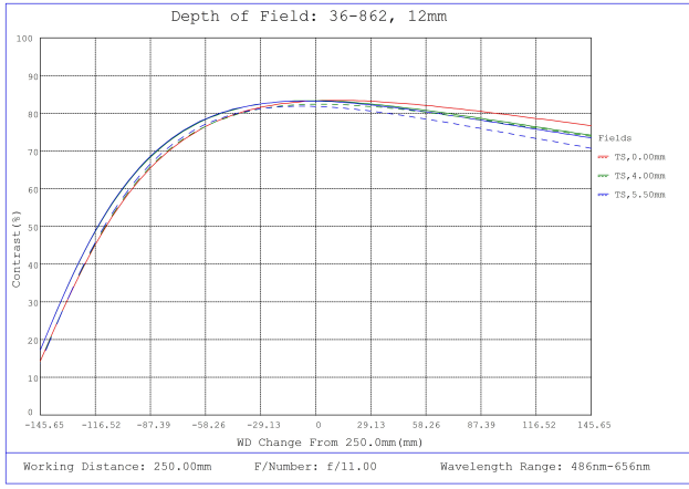
#36-862, 12mm f/11, 150-500mm Primary WD, HRr Series Fixed Focal Length Lens, Depth of Field Plot, 250mm Working Distance, f11
