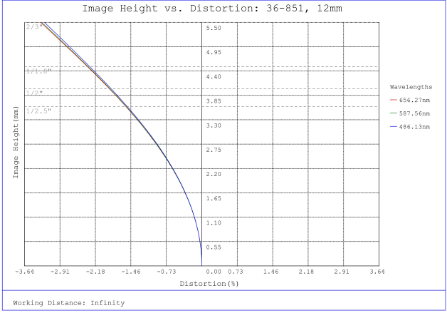
#36-851, 12mm f/2.8, 1000mm-∞ Primary WD, HRr Series Fixed Focal Length Lens, Distortion Plot
