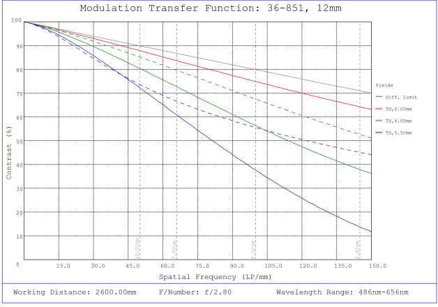
#36-851, 12mm f/2.8, 1000mm-∞ Primary WD, HRr Series Fixed Focal Length Lens, Modulated Transfer Function (MTF) Plot, 2600mm Working Distance, f2.8
