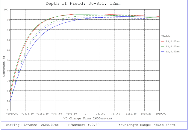
#36-851, 12mm f/2.8, 1000mm-∞ Primary WD, HRr Series Fixed Focal Length Lens, Depth of Field Plot, 2600mm Working Distance, f2.8
