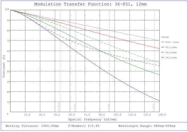
#36-851, 12mm f/2.8, 1000mm-∞ Primary WD, HRr Series Fixed Focal Length Lens, Modulated Transfer Function (MTF) Plot, 1000mm Working Distance, f2.8
