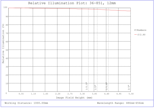
#36-851, 12mm f/2.8, 1000mm-∞ Primary WD, HRr Series Fixed Focal Length Lens, Relative Illumination Plot
