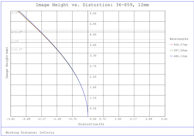
#36-859, 12mm f/8, 400-2000mm Primary WD, HRr Series Fixed Focal Length Lens, Distortion Plot
