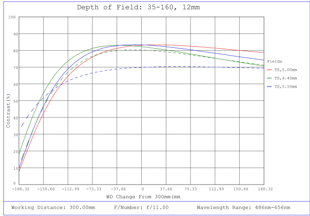
#35-160, 12mm, f/11 Cr Series Fixed Focal Length Lens, Depth of Field Plot, 300mm Working Distance, f11
