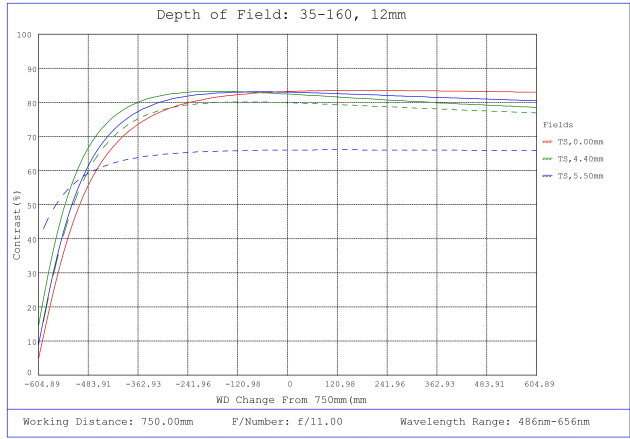
#35-160, 12mm, f/11 Cr Series Fixed Focal Length Lens, Depth of Field Plot, 750mm Working Distance, f11
