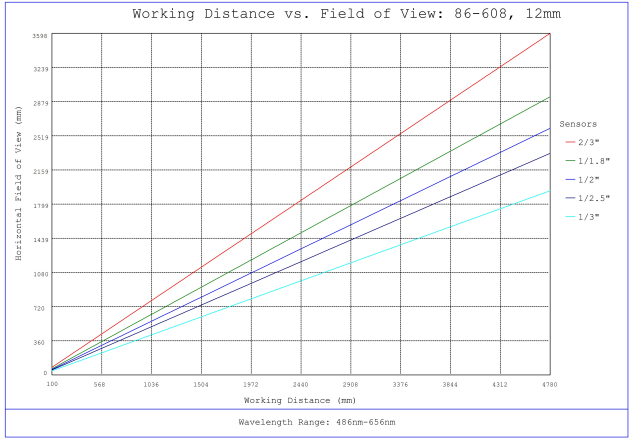
#86-608, 12mm, f/2.8 Ci Series Fixed Focal Length Lens, Working Distance versus Field of View Plot
