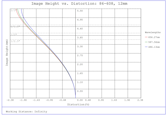
#86-608, 12mm, f/2.8 Ci Series Fixed Focal Length Lens, Distortion Plot
