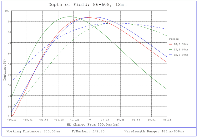
#86-608, 12mm, f/2.8 Ci Series Fixed Focal Length Lens, Depth of Field Plot, 300mm Working Distance, f2.8
