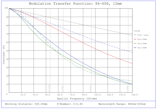
#86-608, 12mm, f/2.8 Ci Series Fixed Focal Length Lens, Modulated Transfer Function (MTF) Plot, 300mm Working Distance, f2.8
