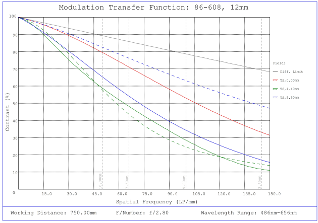
#86-608, 12mm, f/2.8 Ci Series Fixed Focal Length Lens, Modulated Transfer Function (MTF) Plot, 750mm Working Distance, f2.8
