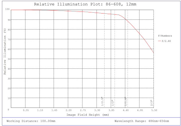
#86-608, 12mm, f/2.8 Ci Series Fixed Focal Length Lens, Relative Illumination Plot
