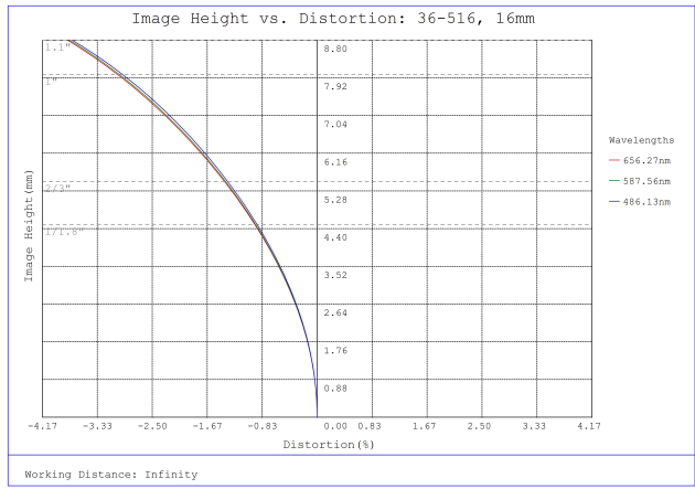
#36-516, 16mm f/11, HPr Series Fixed Focal Length Lens, Distortion Plot
