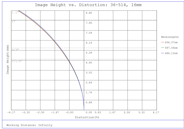
#36-514, 16mm f/5.6, HPr Series Fixed Focal Length Lens, Distortion Plot
