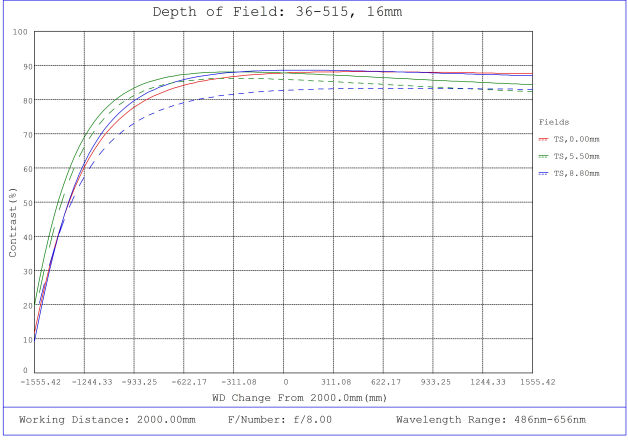
#36-515, 16mm f/8, HPr Series Fixed Focal Length Lens, Depth of Field Plot, 2000mm Working Distance, f8
