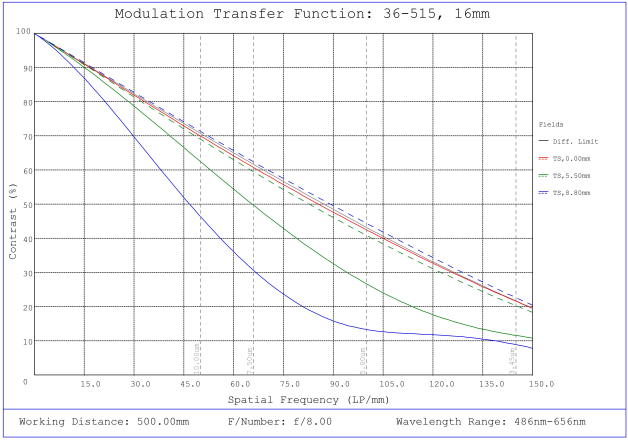
#36-515, 16mm f/8, HPr Series Fixed Focal Length Lens, Modulated Transfer Function (MTF) Plot, 500mm Working Distance, f8
