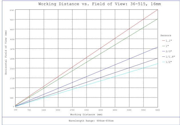
#36-515, 16mm f/8, HPr Series Fixed Focal Length Lens, Working Distance versus Field of View Plot
