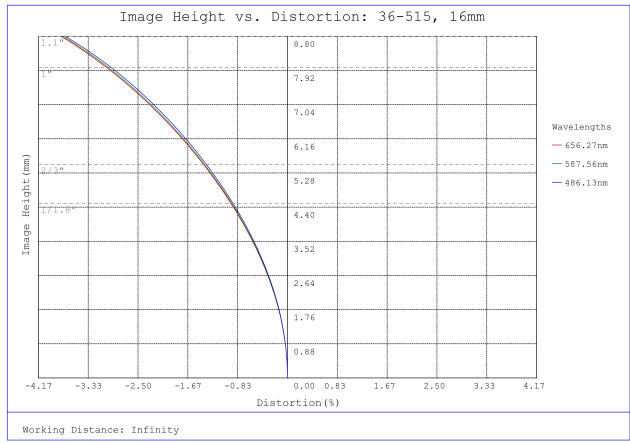
#36-515, 16mm f/8, HPr Series Fixed Focal Length Lens, Distortion Plot
