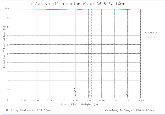
#36-515, 16mm f/8, HPr Series Fixed Focal Length Lens, Relative Illumination Plot
