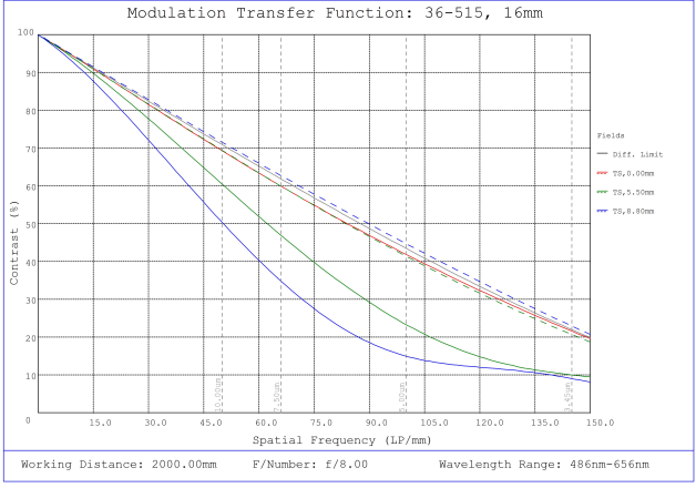
#36-515, 16mm f/8, HPr Series Fixed Focal Length Lens, Modulated Transfer Function (MTF) Plot, 2000mm Working Distance, f8
