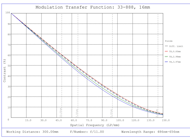
#33-888, 16mm, f/11 UCI Series Fixed Focal Length Lens, Modulated Transfer Function (MTF) Plot, 300mm Working Distance, f11
