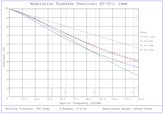
#85-351, 16mm, f/4 Ci Series Fixed Focal Length Lens, Modulated Transfer Function (MTF) Plot, 500mm Working Distance, f4
