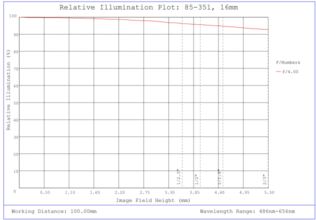
#85-351, 16mm, f/4 Ci Series Fixed Focal Length Lens, Relative Illumination Plot
