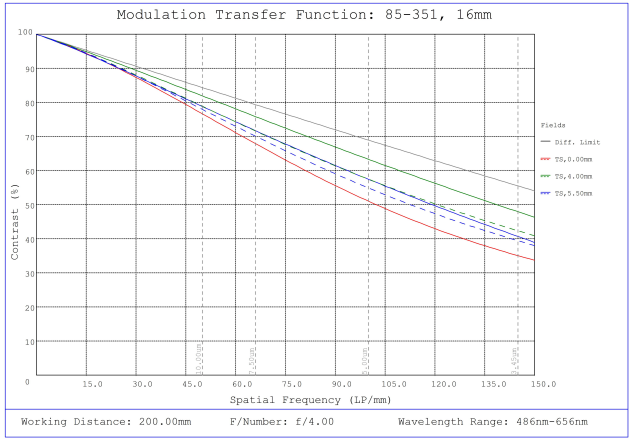
#85-351, 16mm, f/4 Ci Series Fixed Focal Length Lens, Modulated Transfer Function (MTF) Plot, 200mm Working Distance, f4
