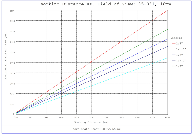
#85-351, 16mm, f/4 Ci Series Fixed Focal Length Lens, Working Distance versus Field of View Plot
