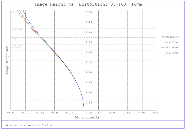
#35-168, 16mm, f/8 Cr Series Fixed Focal Length Lens, Distortion Plot
