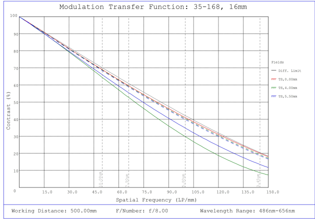
#35-168, 16mm, f/8 Cr Series Fixed Focal Length Lens, Modulated Transfer Function (MTF) Plot, 500mm Working Distance, f8
