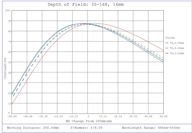
#35-168, 16mm, f/8 Cr Series Fixed Focal Length Lens, Depth of Field Plot, 200mm Working Distance, f8
