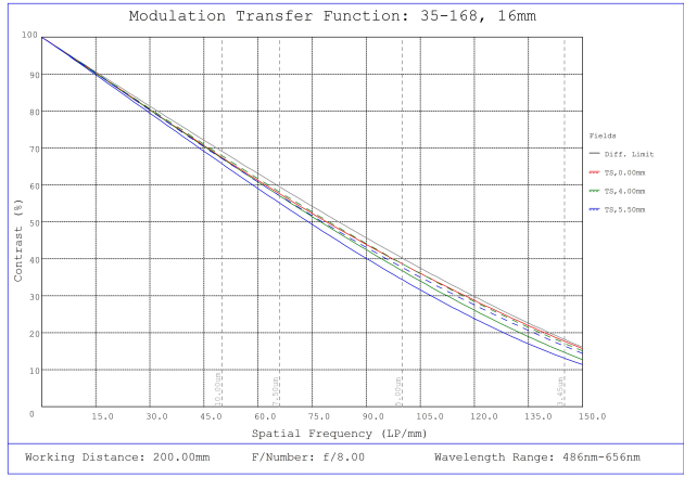
#35-168, 16mm, f/8 Cr Series Fixed Focal Length Lens, Modulated Transfer Function (MTF) Plot, 200mm Working Distance, f8
