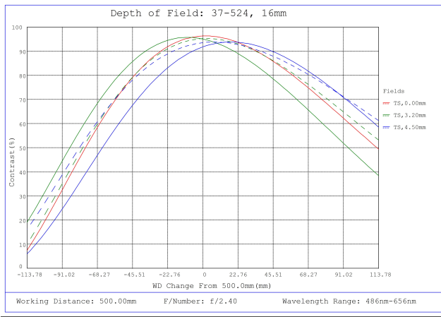
#37-524, 16mm FL, Liquid Lens M12 Lens, Depth of Field Plot, 500mm Working Distance, f2.4
