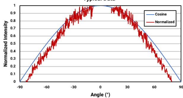
Typical, normalized reflectance profile of Optopolymer®, showing near Lambertian properties. The gap in data is due to the detector crossing the path of the incident beam.
