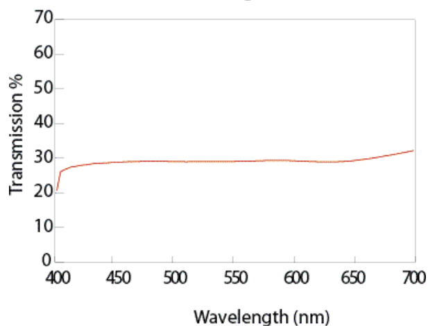
Transmission for Single Glass Polarizer
