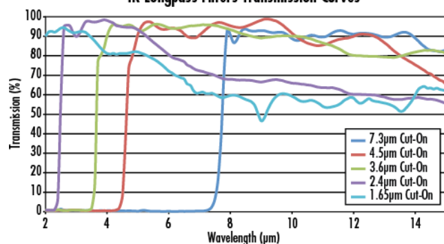
IR Longpass Filters Transmission Curves
