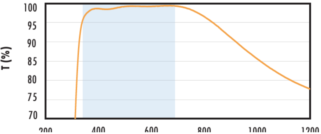
Fused Silica with VIS-EXT Coating Typical Transmission
