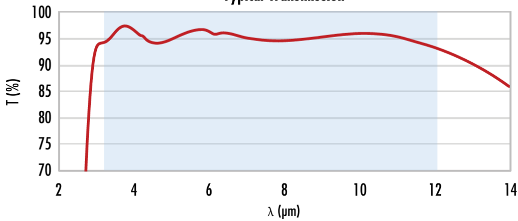
ZnSe with 3-12 microns AR Coating Typical Transmission
