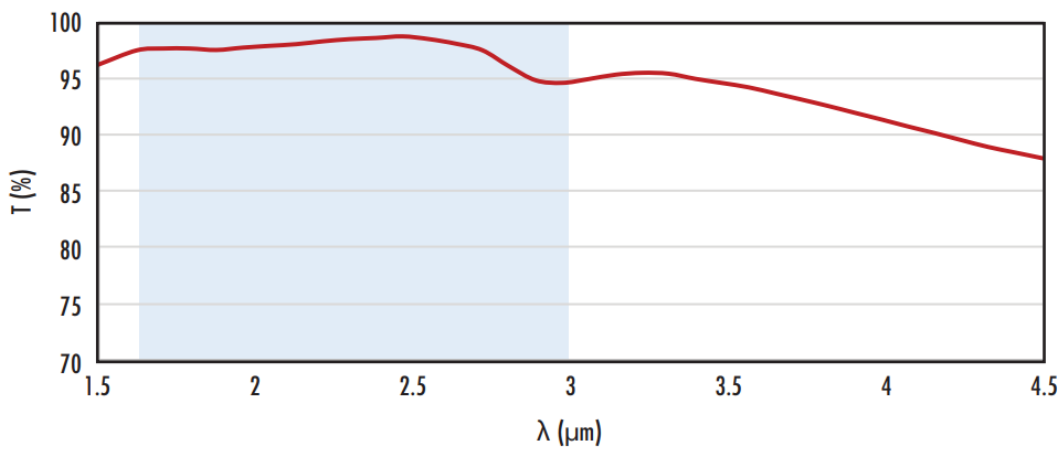
ZnSe with 1.65-3 microns AR Coating Typical Transmission
