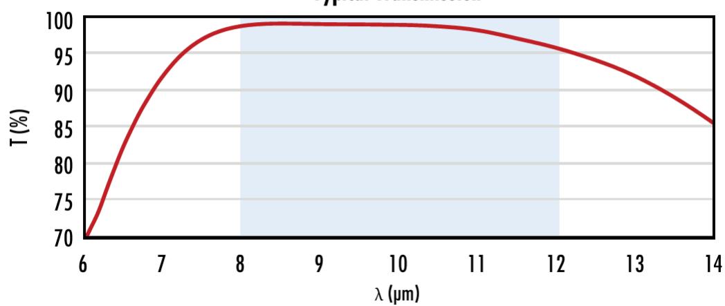
ZnSe with 8-12 microns AR Coating Typical Transmission
