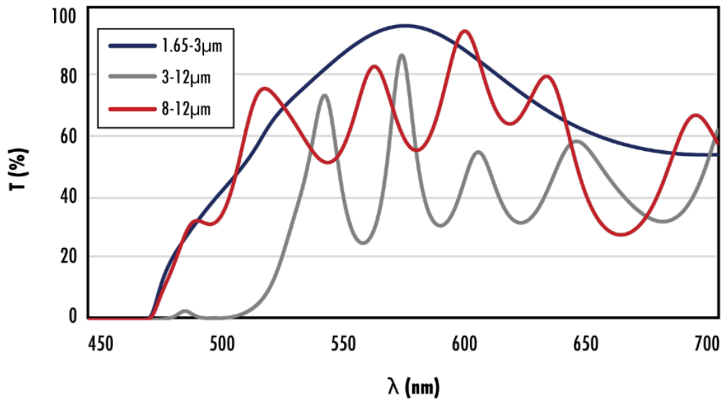
ZnSe with 1.65-3 microns AR Coating Typical Transmission
