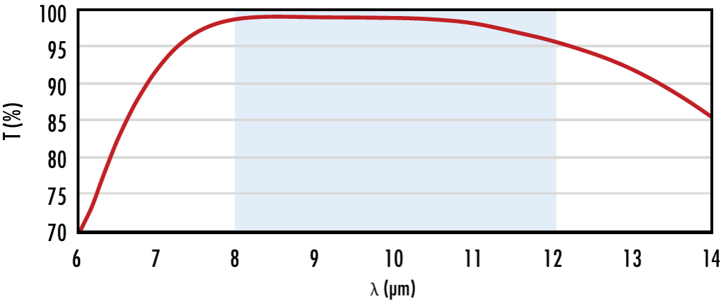
ZnSe with 8-12 \mu m AR Coating Typical Transmission
