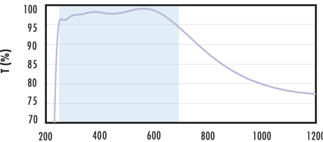
Fused Silica with UV-VIS Coating Typical Transmission
