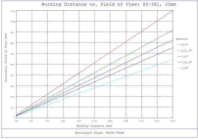
#85-361, 25mm, f/11 Ci Series Fixed Focal Length Lens, Working Distance versus Field of View Plot
