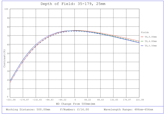
#35-179, 25mm, f/16 Cr Series Fixed Focal Length Lens, Depth of Field Plot, 500mm Working Distance, f16
