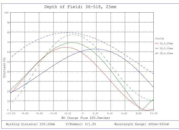
#36-518, 25mm f/1.8, HPr Series Fixed Focal Length Lens, Depth of Field Plot, 200mm Working Distance, f1.8
