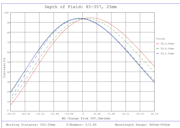
#85-357, 25mm, f/2.8 Ci Series Fixed Focal Length Lens, Depth of Field Plot, 500mm Working Distance, f2.8
