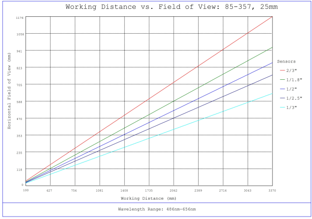
#85-357, 25mm, f/2.8 Ci Series Fixed Focal Length Lens, Working Distance versus Field of View Plot
