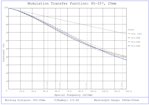
#85-357, 25mm, f/2.8 Ci Series Fixed Focal Length Lens, Modulated Transfer Function (MTF) Plot, 500mm Working Distance, f2.8
