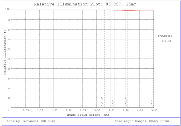
#85-357, 25mm, f/2.8 Ci Series Fixed Focal Length Lens, Relative Illumination Plot
