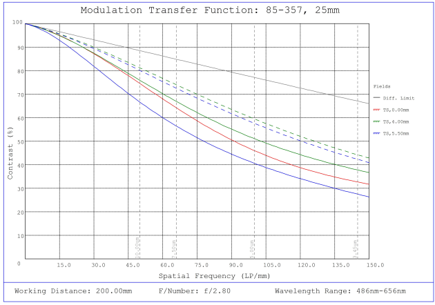
#85-357, 25mm, f/2.8 Ci Series Fixed Focal Length Lens, Modulated Transfer Function (MTF) Plot, 200mm Working Distance, f2.8
