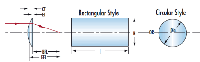
Circular And Rectangular Cylinder Lenses
