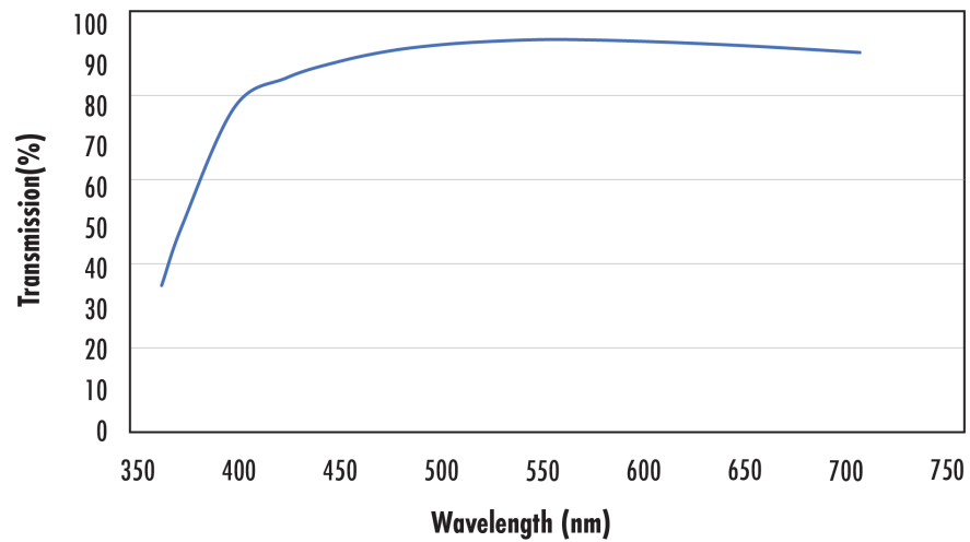
#15-940 Reference Transmission Plot
