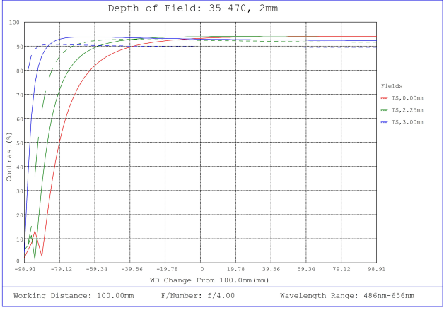
#35-470, 2mm FL f/4 IR-Cut Rugged Blue Series M12 Lens, Depth of Field Plot, 100mm Working Distance, f4
