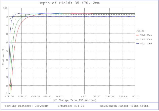
#35-470, 2mm FL f/4 IR-Cut Rugged Blue Series M12 Lens, Depth of Field Plot, 250mm Working Distance, f4
