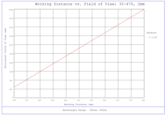
#35-470, 2mm FL f/4 IR-Cut Rugged Blue Series M12 Lens, Working Distance versus Field of View Plot
