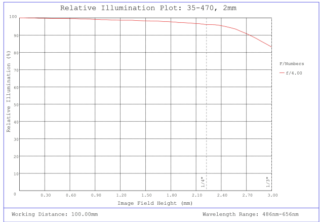
#35-470, 2mm FL f/4 IR-Cut Rugged Blue Series M12 Lens, Relative Illumination Plot
