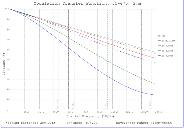
#35-470, 2mm FL f/4 IR-Cut Rugged Blue Series M12 Lens, Modulated Transfer Function (MTF) Plot, 250mm Working Distance, f4
