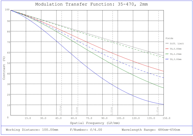
#35-470, 2mm FL f/4 IR-Cut Rugged Blue Series M12 Lens, Modulated Transfer Function (MTF) Plot, 100mm Working Distance, f4
