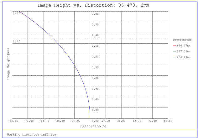
#35-470, 2mm FL f/4 IR-Cut Rugged Blue Series M12 Lens, Distortion Plot
