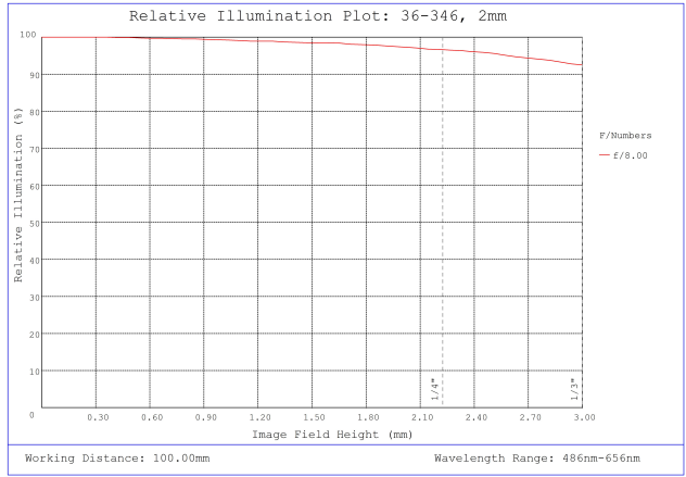
#36-346, 2mm FL f/8 Rugged Blue Series M12 Lens, Relative Illumination Plot
