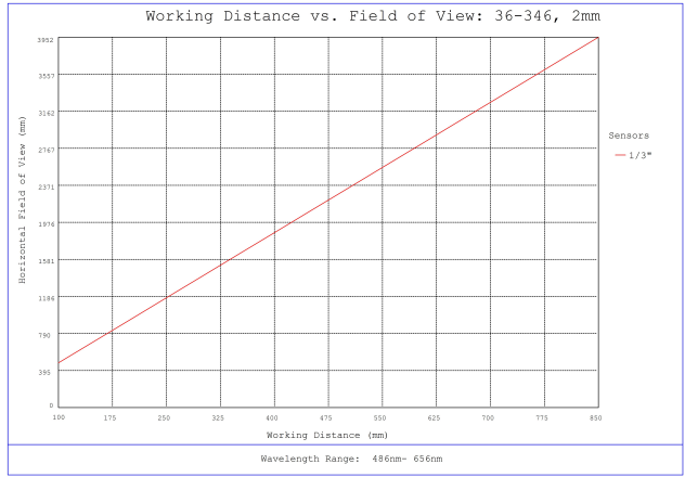
#36-346, 2mm FL f/8 Rugged Blue Series M12 Lens, Working Distance versus Field of View Plot
