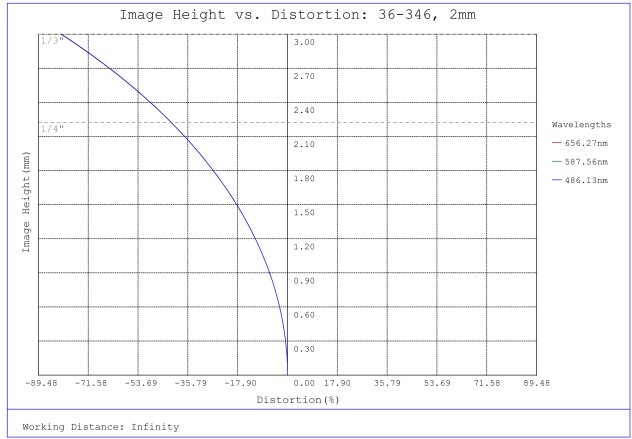
#36-346, 2mm FL f/8 Rugged Blue Series M12 Lens, Distortion Plot
