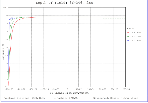
#36-346, 2mm FL f/8 Rugged Blue Series M12 Lens, Depth of Field Plot, 250mm Working Distance, f8
