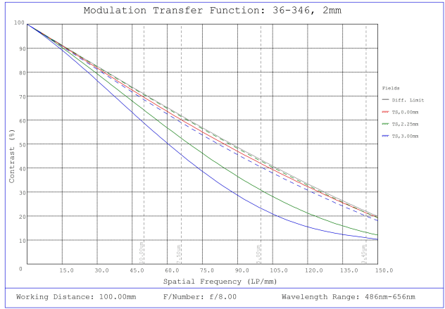
#36-346, 2mm FL f/8 Rugged Blue Series M12 Lens, Modulated Transfer Function (MTF) Plot, 100mm Working Distance, f8
