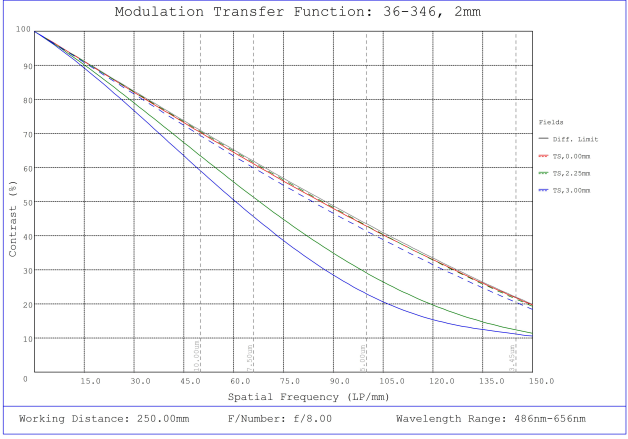
#36-346, 2mm FL f/8 Rugged Blue Series M12 Lens, Modulated Transfer Function (MTF) Plot, 250mm Working Distance, f8
