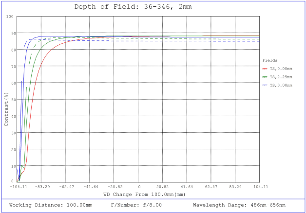
#36-346, 2mm FL f/8 Rugged Blue Series M12 Lens, Depth of Field Plot, 100mm Working Distance, f8
