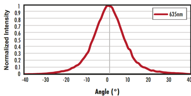
Relative Intensity vs. Angle Light Diffusing Film
