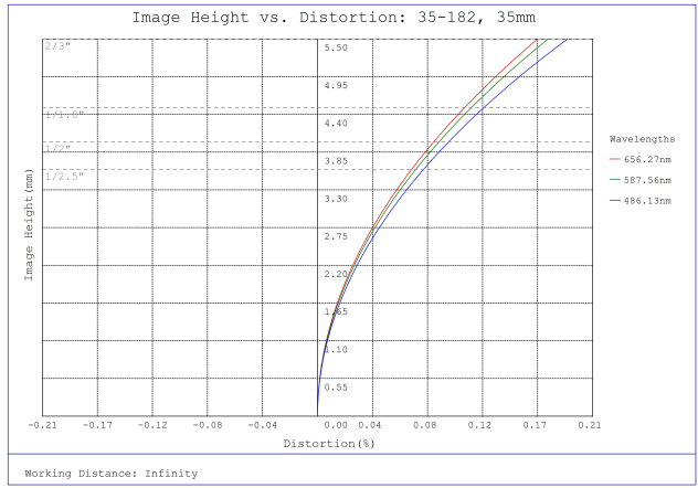
#35-182, 35mm, f/1.8 Cr Series Fixed Focal Length Lens, Distortion Plot
