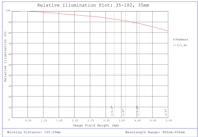
#35-182, 35mm, f/1.8 Cr Series Fixed Focal Length Lens, Relative Illumination Plot
