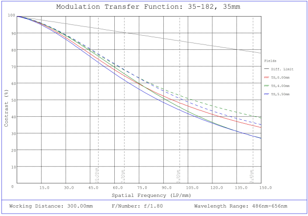
#35-182, 35mm, f/1.8 Cr Series Fixed Focal Length Lens, Modulated Transfer Function (MTF) Plot, 300mm Working Distance, f1.8
