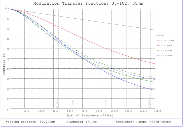
#35-182, 35mm, f/1.8 Cr Series Fixed Focal Length Lens, Modulated Transfer Function (MTF) Plot, 500mm Working Distance, f1.8
