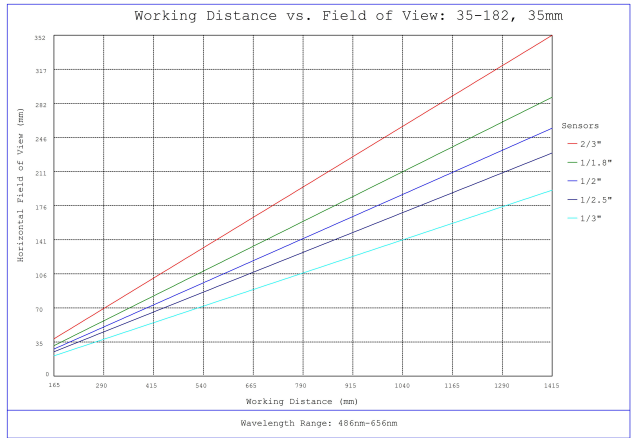
#35-182, 35mm, f/1.8 Cr Series Fixed Focal Length Lens, Working Distance versus Field of View Plot
