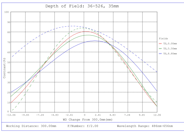
#36-526, 35mm f/2.0, HPr Series Fixed Focal Length Lens, Depth of Field Plot, 300mm Working Distance, f2
