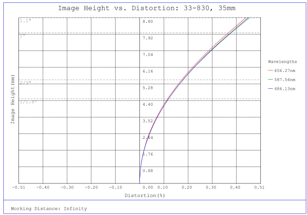
#33-830, 35mm f/2.8, HPi Series Fixed Focal Length Lens, Distortion Plot
