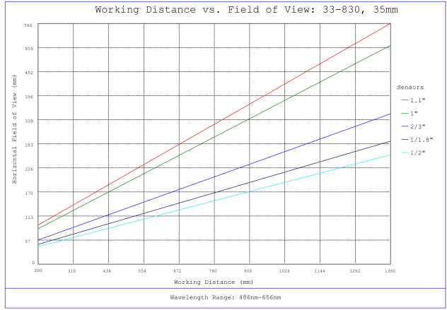
#33-830, 35mm f/2.8, HPi Series Fixed Focal Length Lens, Working Distance versus Field of View Plot
