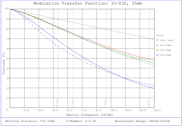
#33-830, 35mm f/2.8, HPi Series Fixed Focal Length Lens, Modulated Transfer Function (MTF) Plot, 750mm Working Distance, f2.8
