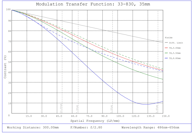
#33-830, 35mm f/2.8, HPi Series Fixed Focal Length Lens, Modulated Transfer Function (MTF) Plot, 300mm Working Distance, f2.8
