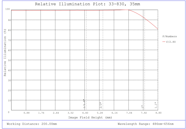
#33-830, 35mm f/2.8, HPi Series Fixed Focal Length Lens, Relative Illumination Plot
