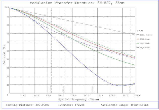
#36-527, 35mm f/2.8, HPr Series Fixed Focal Length Lens, Modulated Transfer Function (MTF) Plot, 300mm Working Distance, f2.8
