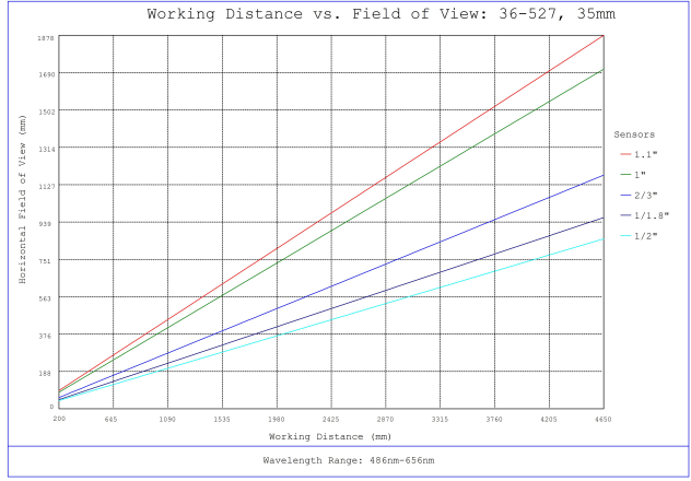
#36-527, 35mm f/2.8, HPr Series Fixed Focal Length Lens, Working Distance versus Field of View Plot
