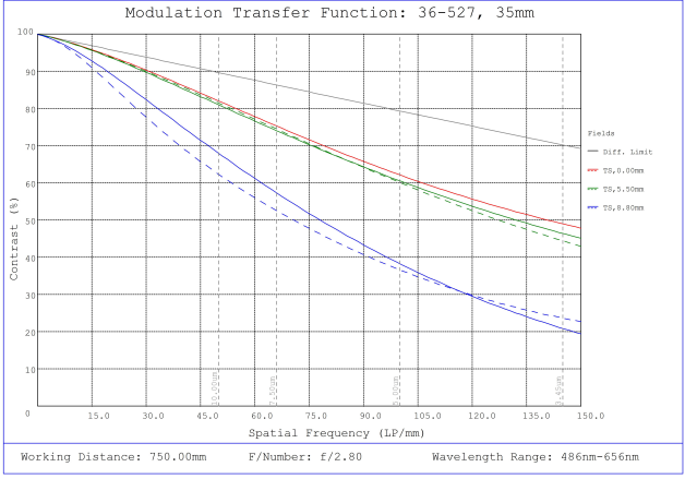
#36-527, 35mm f/2.8, HPr Series Fixed Focal Length Lens, Modulated Transfer Function (MTF) Plot, 750mm Working Distance, f2.8
