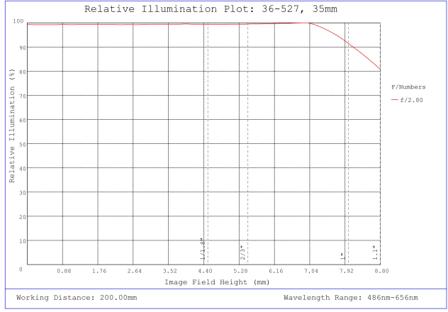
#36-527, 35mm f/2.8, HPr Series Fixed Focal Length Lens, Relative Illumination Plot
