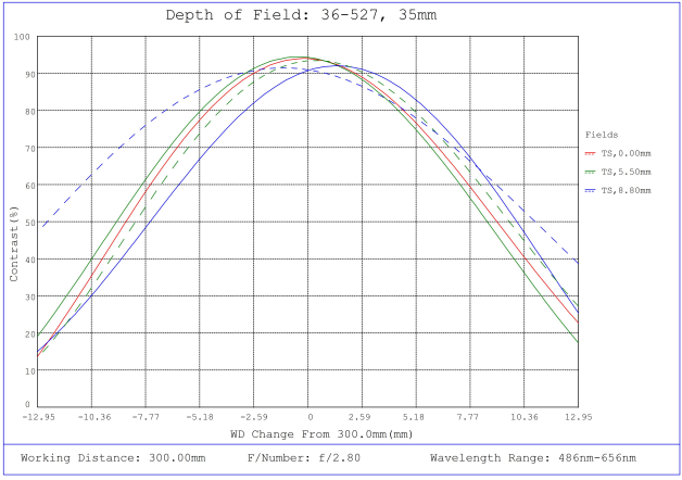
#36-527, 35mm f/2.8, HPr Series Fixed Focal Length Lens, Depth of Field Plot, 300mm Working Distance, f2.8
