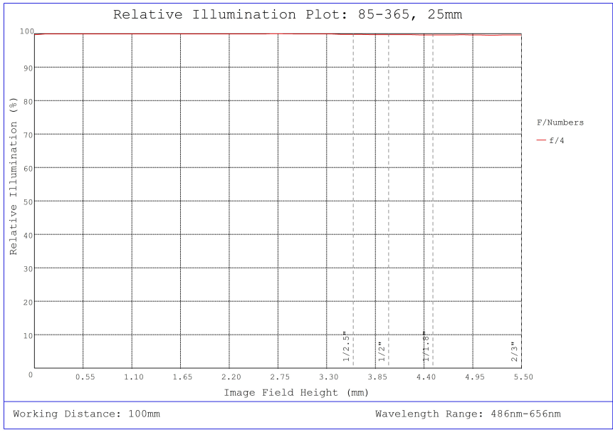
#85-365, 35mm, f/4 Ci Series Fixed Focal Length Lens, Relative Illumination Plot
