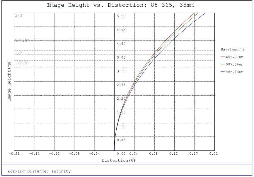
#85-365, 35mm, f/4 Ci Series Fixed Focal Length Lens, Distortion Plot
