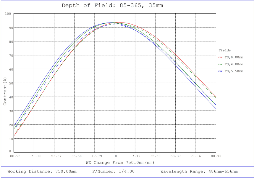
#85-365, 35mm, f/4 Ci Series Fixed Focal Length Lens, Depth of Field Plot, 750mm Working Distance, f4
