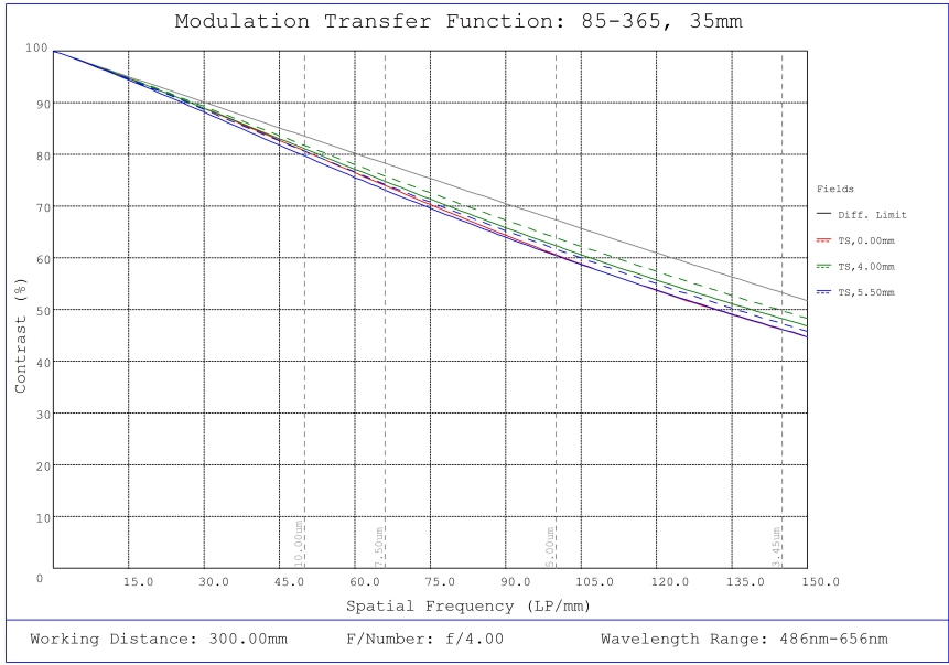
#85-365, 35mm, f/4 Ci Series Fixed Focal Length Lens, Modulated Transfer Function (MTF) Plot, 300mm Working Distance, f4
