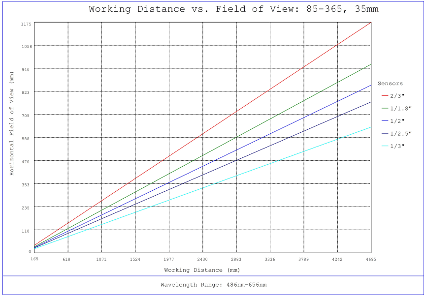
#85-365, 35mm, f/4 Ci Series Fixed Focal Length Lens, Working Distance versus Field of View Plot
