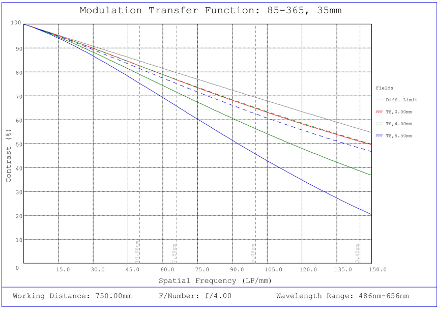
#85-365, 35mm, f/4 Ci Series Fixed Focal Length Lens, Modulated Transfer Function (MTF) Plot, 750mm Working Distance, f4
