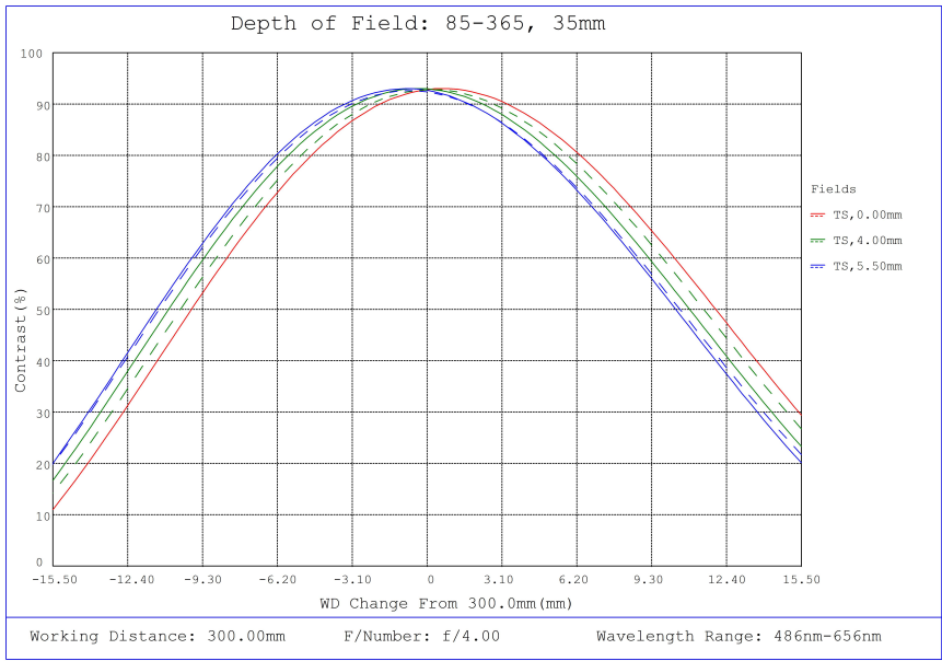
#85-365, 35mm, f/4 Ci Series Fixed Focal Length Lens, Depth of Field Plot, 300mm Working Distance, f4
