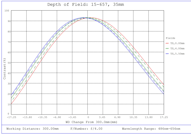
#15-657, 35mm, f/4 Cw Series Fixed Focal Length Lens, Depth of Field Plot, 300mm Working Distance, f4
