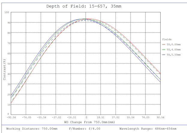
#15-657, 35mm, f/4 Cw Series Fixed Focal Length Lens, Depth of Field Plot, 750mm Working Distance, f4
