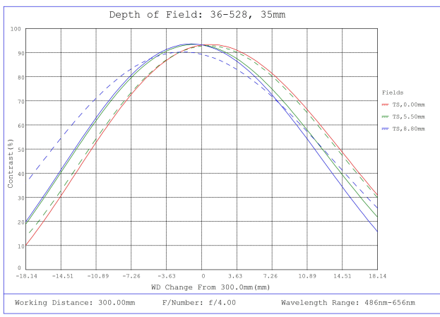
#36-528, 35mm f/4.0, HPr Series Fixed Focal Length Lens, Depth of Field Plot, 300mm Working Distance, f4
