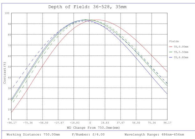
#36-528, 35mm f/4.0, HPr Series Fixed Focal Length Lens, Depth of Field Plot, 750mm Working Distance, f4
