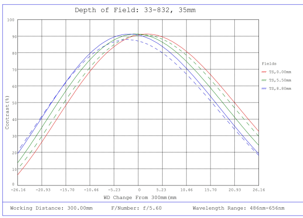
#33-832, 35mm f/5.6, HPI Series Fixed Focal Length Lens, Depth of Field Plot, 300mm Working Distance, f5.6
