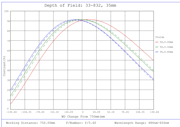
#33-832, 35mm f/5.6, HPI Series Fixed Focal Length Lens, Depth of Field Plot, 750mm Working Distance, f5.6
