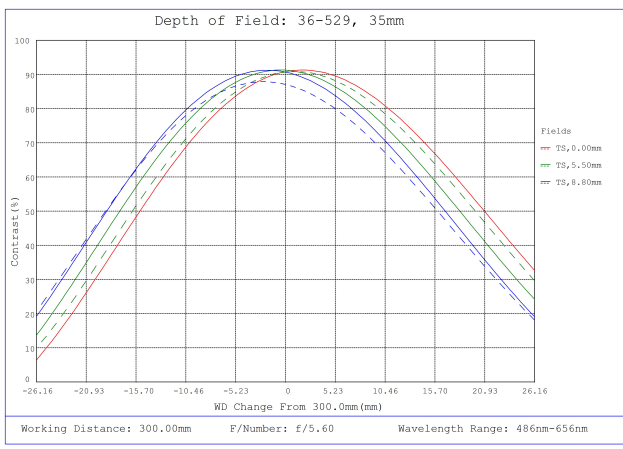
#36-529, 35mm f/5.6, HPr Series Fixed Focal Length Lens, Depth of Field Plot, 300mm Working Distance, f5.6
