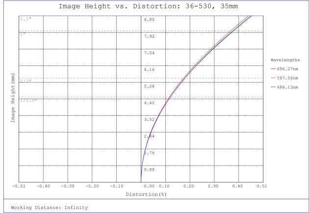
#36-530, 35mm f/8.0, HPr Series Fixed Focal Length Lens, Distortion Plot
