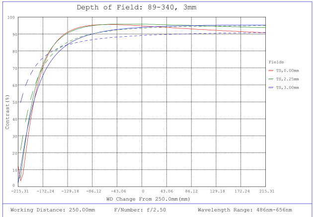
#89-340, 3mm FL f/2.5, Blue Series M12 Lens, Depth of Field Plot, 250mm Working Distance, f2.5
