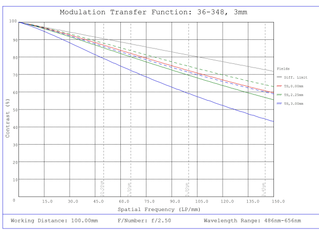
#36-348, 3mm FL f/2.5, Rugged Blue Series M12 Lens, Modulated Transfer Function (MTF) Plot, 100mm Working Distance, f2.5
