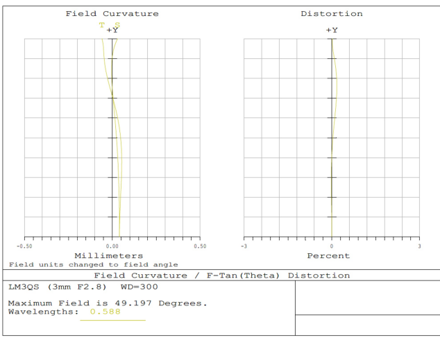
3mm FL, f/2.8, Low Distortion M12 Lens, Distortion Plot
